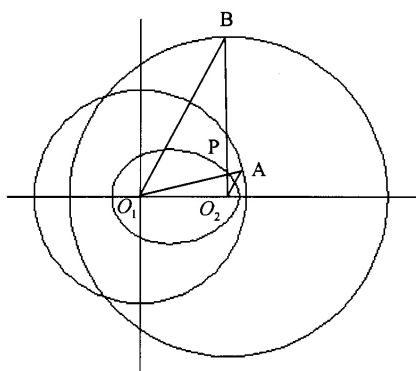
Figure 5: Descartes' oval curves
